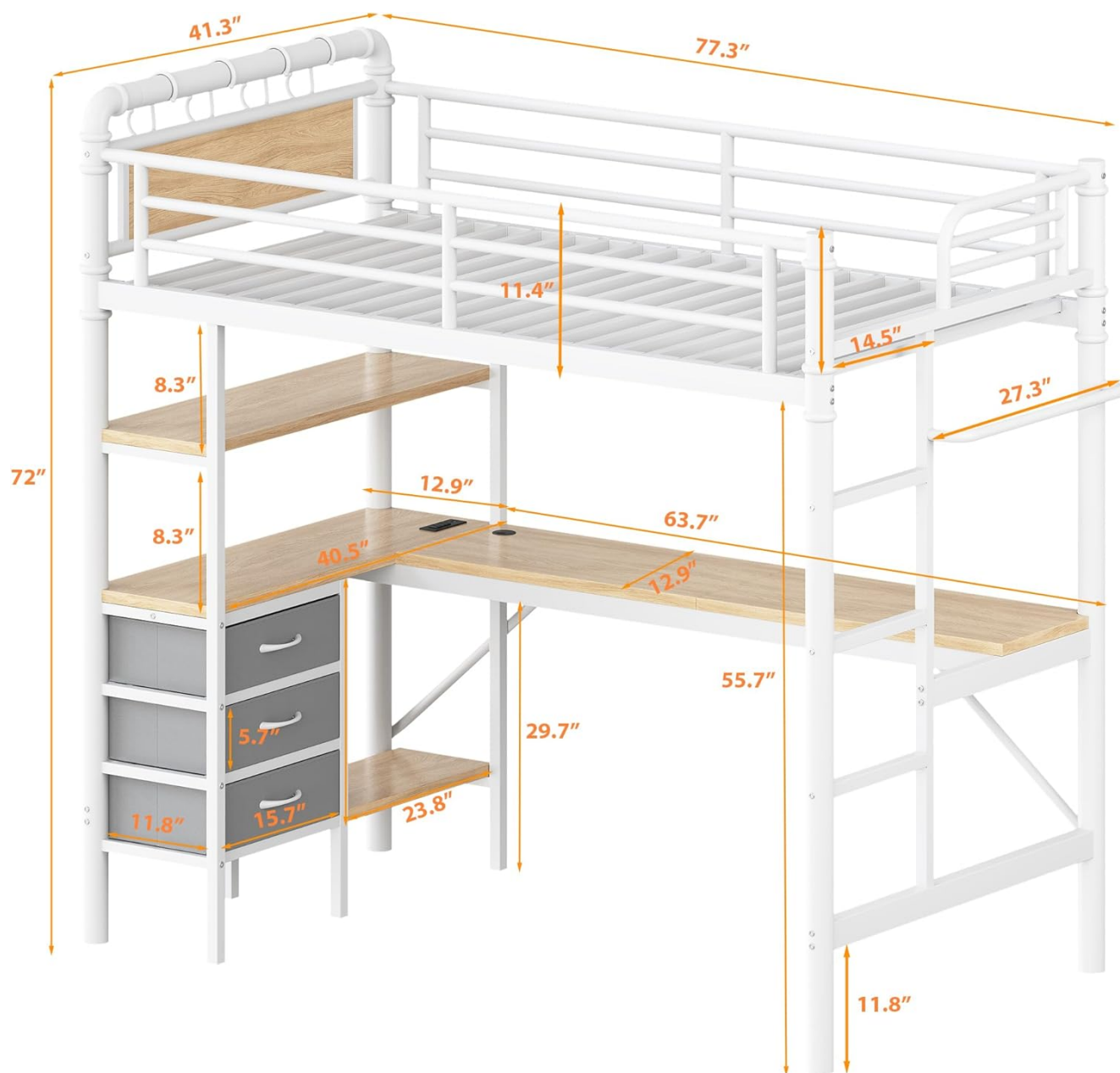
Figure 9.1: Detailed dimensions of the Jocoevol Twin Size Loft Bed, including overall length, width, height, and specific measurements for the desk, shelves, and bed clearance.
