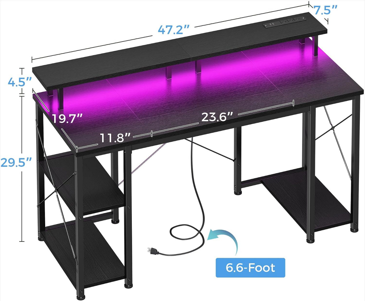
Image: Dimensional diagram of the ODK 48-inch gaming desk, indicating key measurements.
