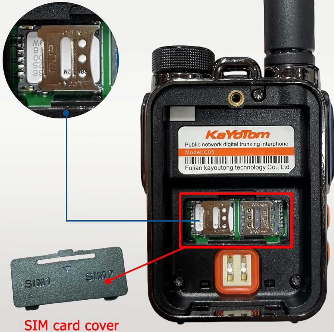
Image 3.2: SIM card slot location and cover.
