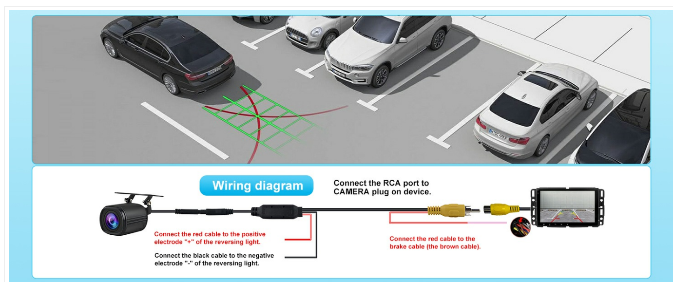
Figure 5: Rear camera wiring instructions.
