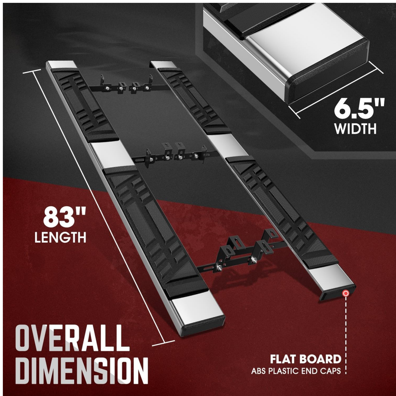
Figure 5: Overall dimensions of the running boards.
