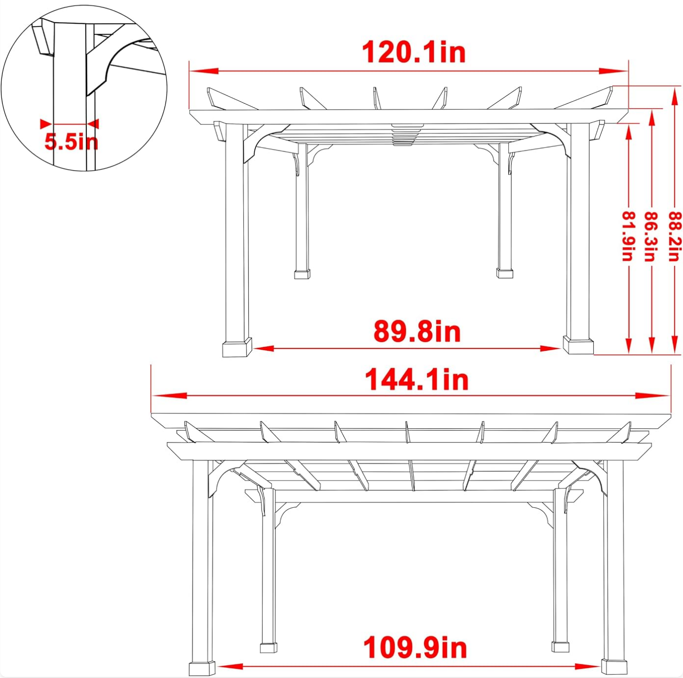
Image 3.1: Detailed dimensions of the pergola, including post and interior measurements.
