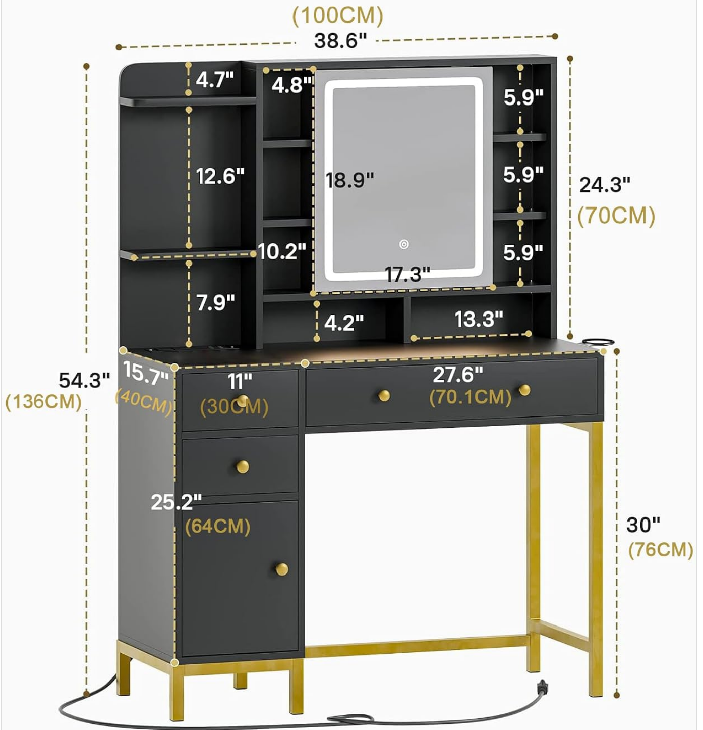
Image 8.1: Detailed dimensional diagram of the KINKUNCO Vanity, Model H01, indicating key measurements.
