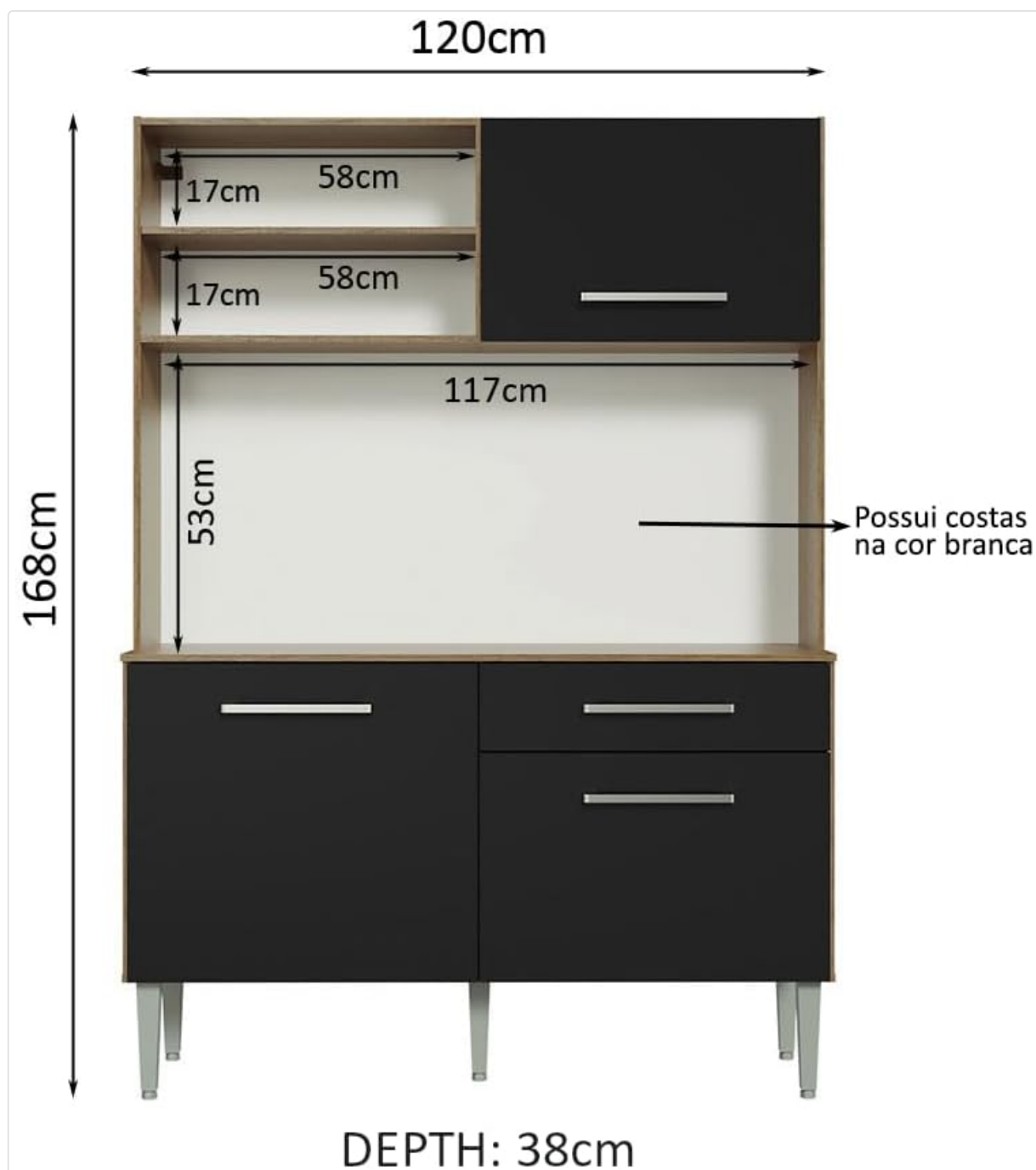
Image 3.1: Dimensional drawing of the Madesa Life Compact Kitchen Cabinet. This diagram illustrates the overall height (168cm), width (120cm), and depth (38cm), along with internal shelf and compartment measurements.
