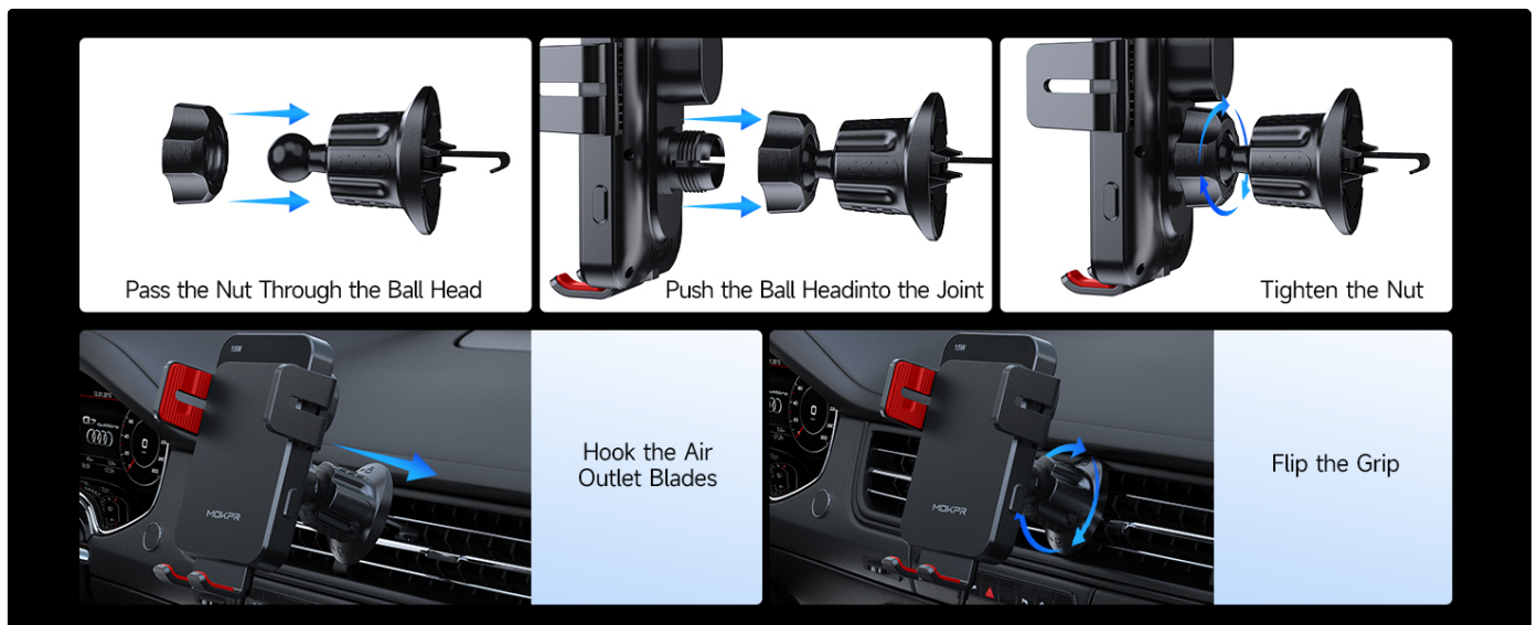
Image 4.1: Visual guide for installing the suction cup mount on a dashboard, showing cleaning, attaching, and securing steps.
