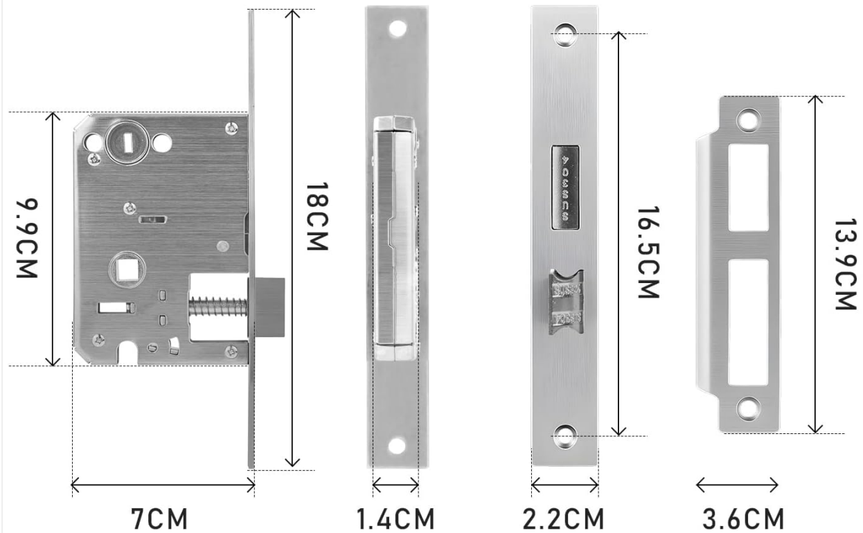
Figure 4.1: Lock cylinder dimensions and measurements for door preparation.
