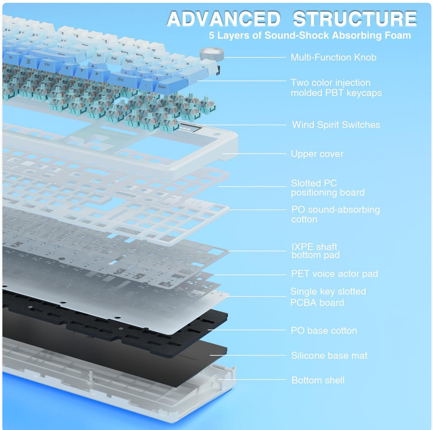
Figure 6: Internal Structure with Sound-Dampening Layers.
