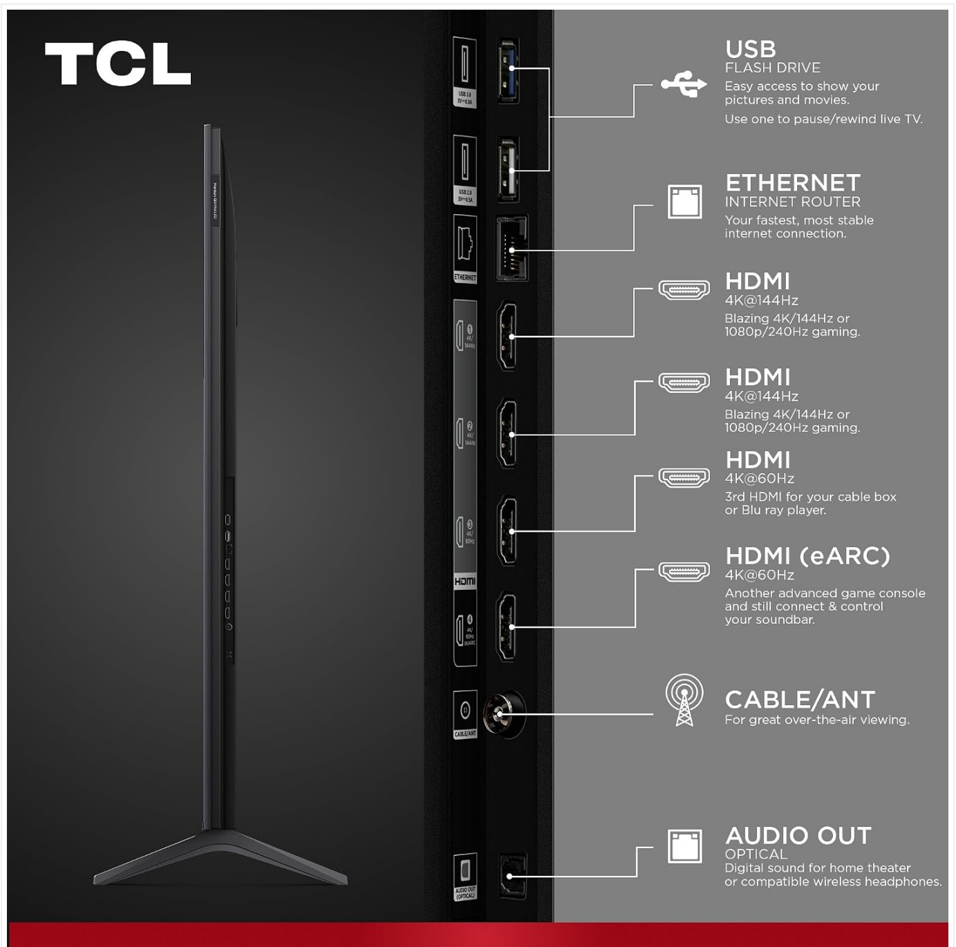
Image: A detailed view of the side and rear connectivity ports on the TCL 55QM6K TV, including USB, Ethernet, multiple HDMI inputs (including eARC), Cable/Antenna, and Optical Audio Out.
