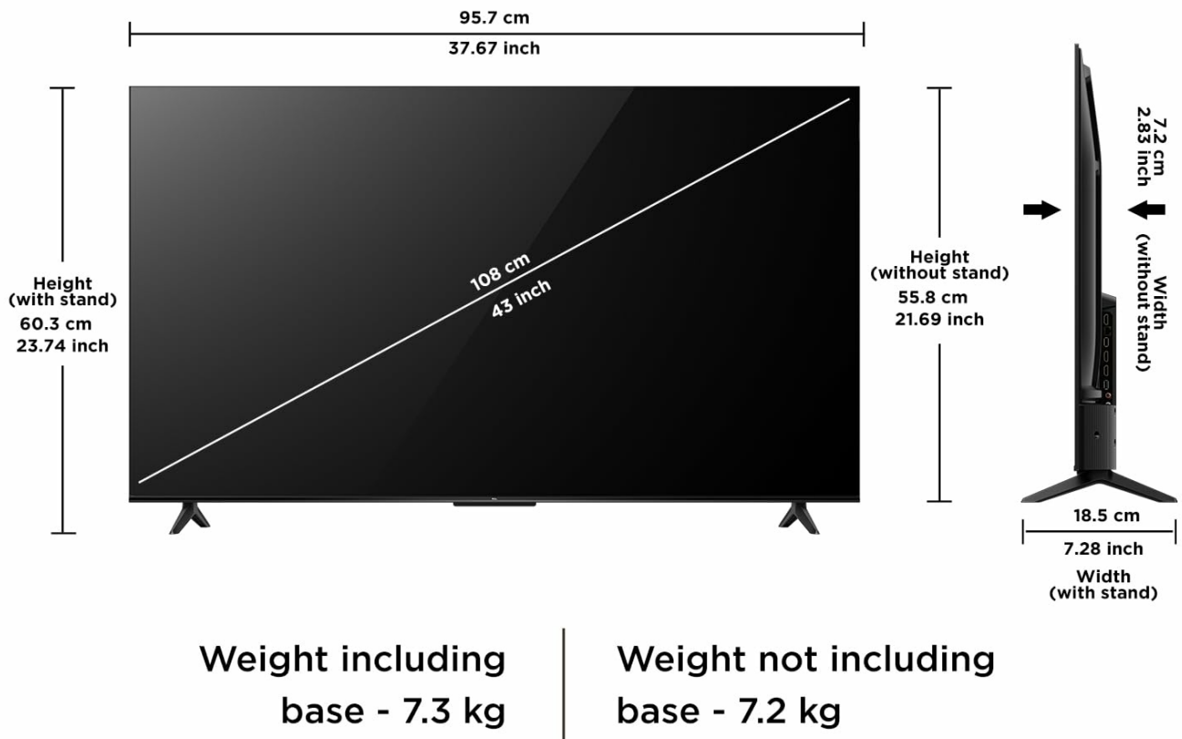
Figure 2.3: TV dimensions for installation planning.
