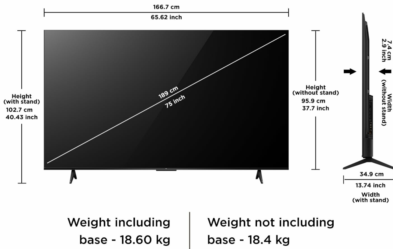
Image 3.1: Detailed dimensions of the TCL 75V6C television, including height, width, and depth with and without the stand, along with weight specifications.
