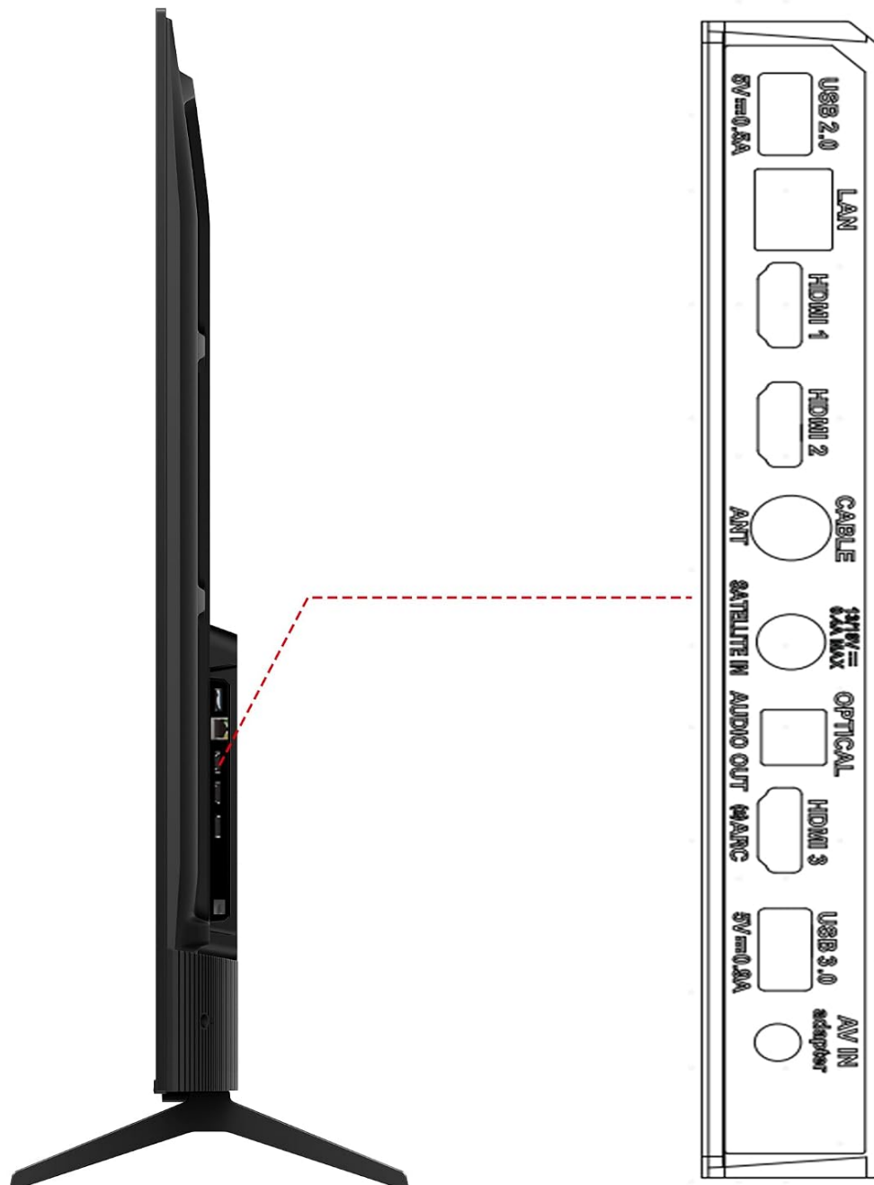
Image 3.2: Side view of the TCL 75V6C TV illustrating the location and types of input/output ports, including USB, LAN, HDMI, Satellite In, Optical Audio Out, and AV In.
