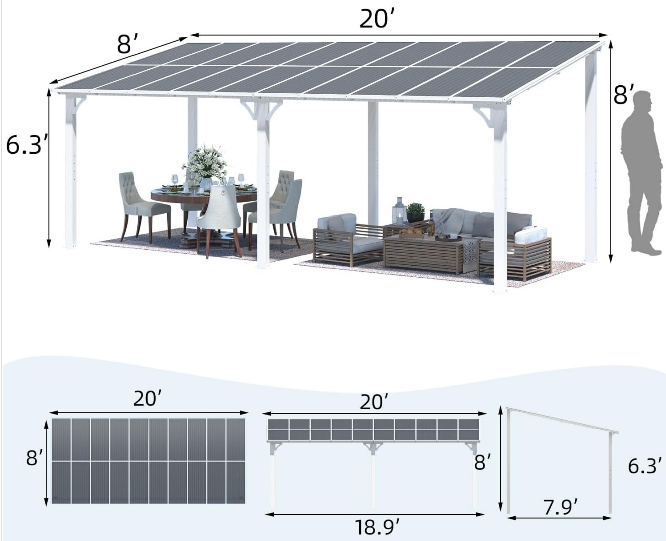
Image: A detailed diagram illustrating the overall dimensions and key measurements of the 20' x 8' hardtop gazebo.
