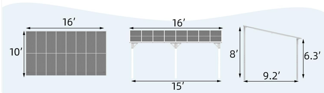
Image 8.1: Detailed dimensions of the AECOJOY 16' x 10' Hardtop Gazebo.
