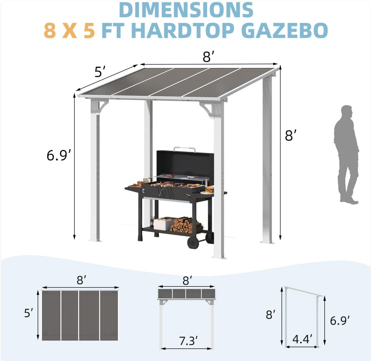
Dimensional diagram of the AECOJOY 8' x 5' Gazebo.
