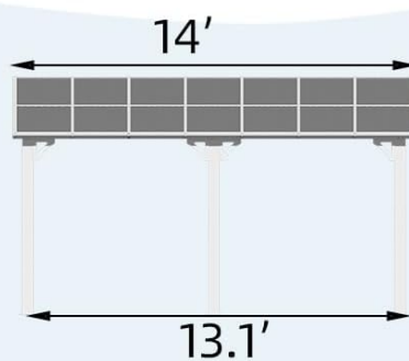
Dimensional diagram of the AECOJOY 14' x 8' Hardtop Gazebo.
