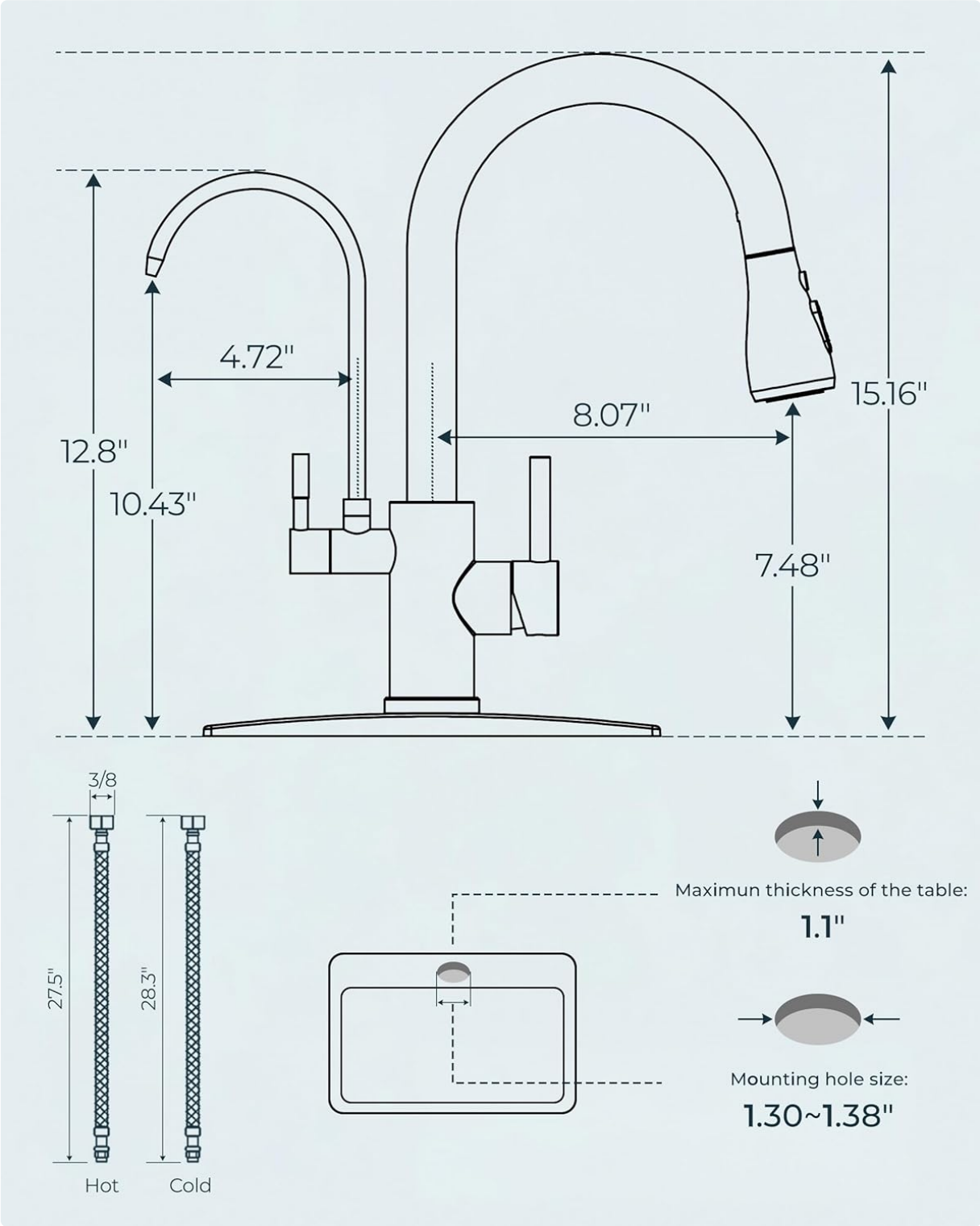
Image: Detailed diagram showing the dimensions of the FORIOUS Kitchen Faucet.
