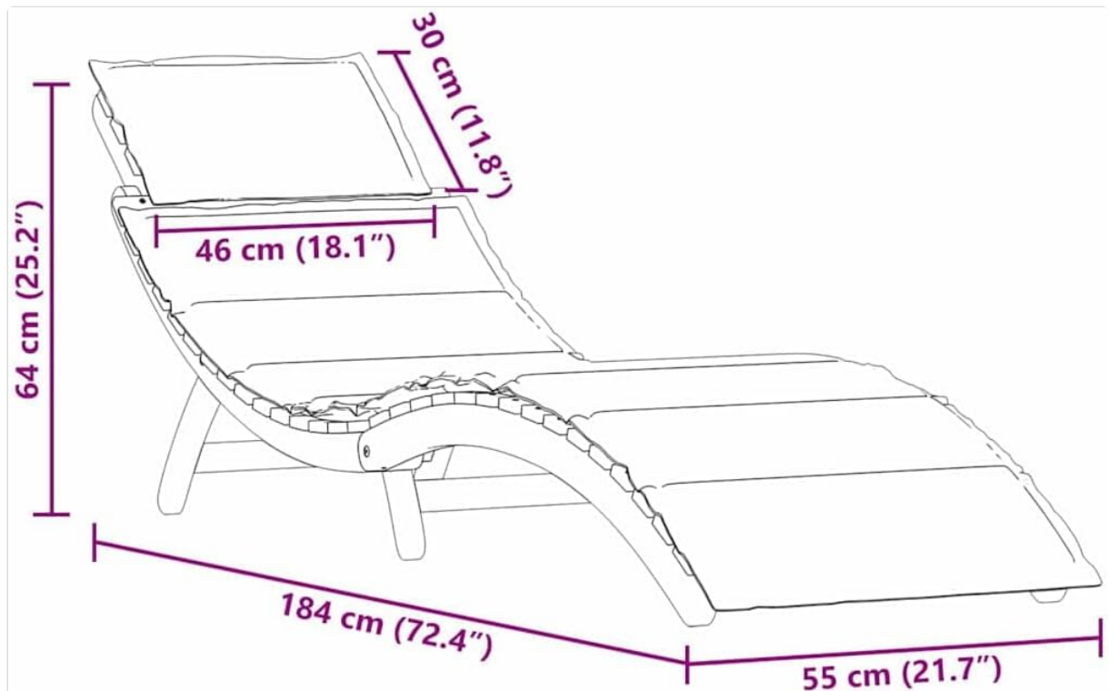
Image: A detailed dimension diagram of the sun lounger.
