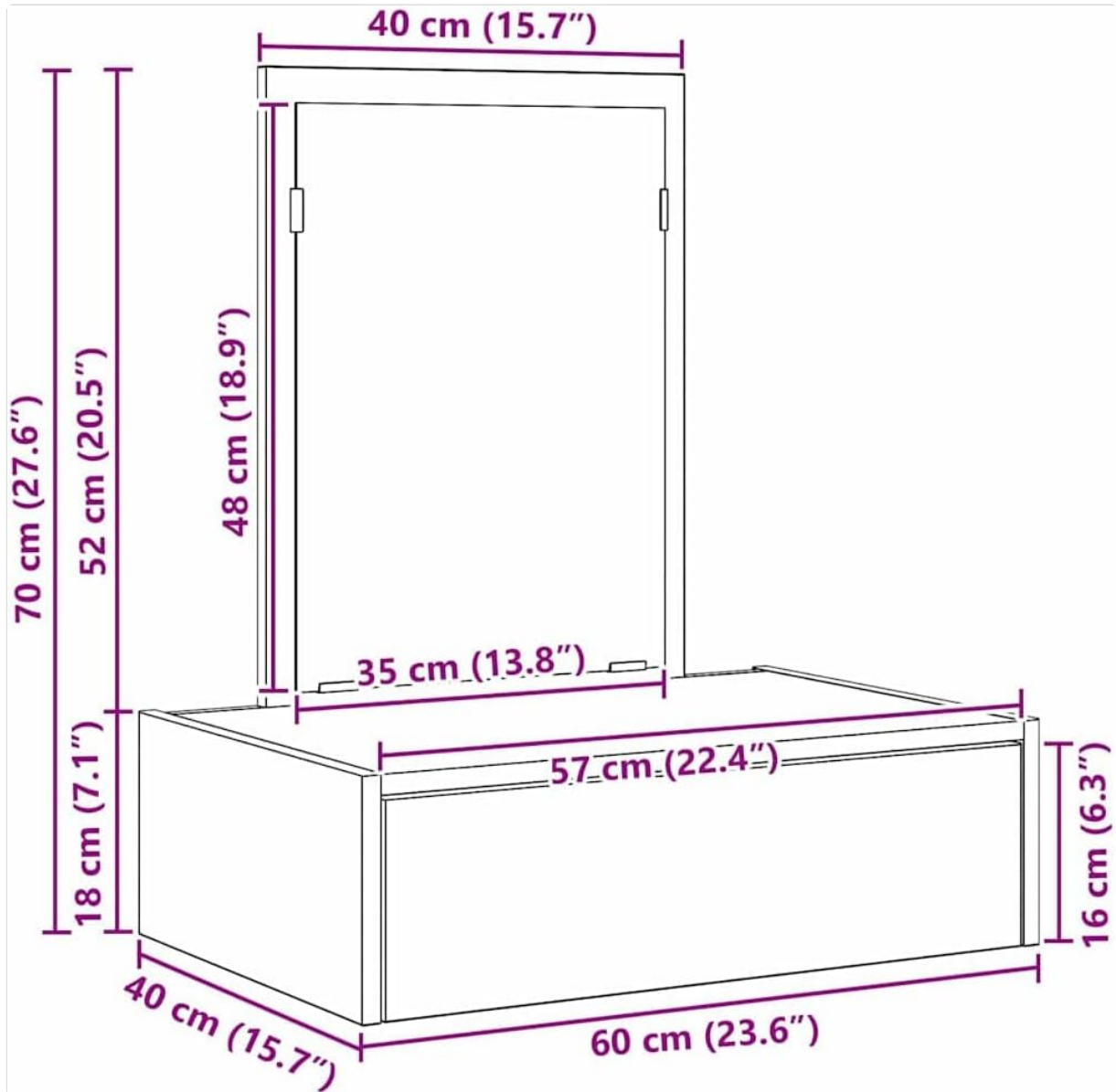
Image 4.1: Product dimensions diagram.
