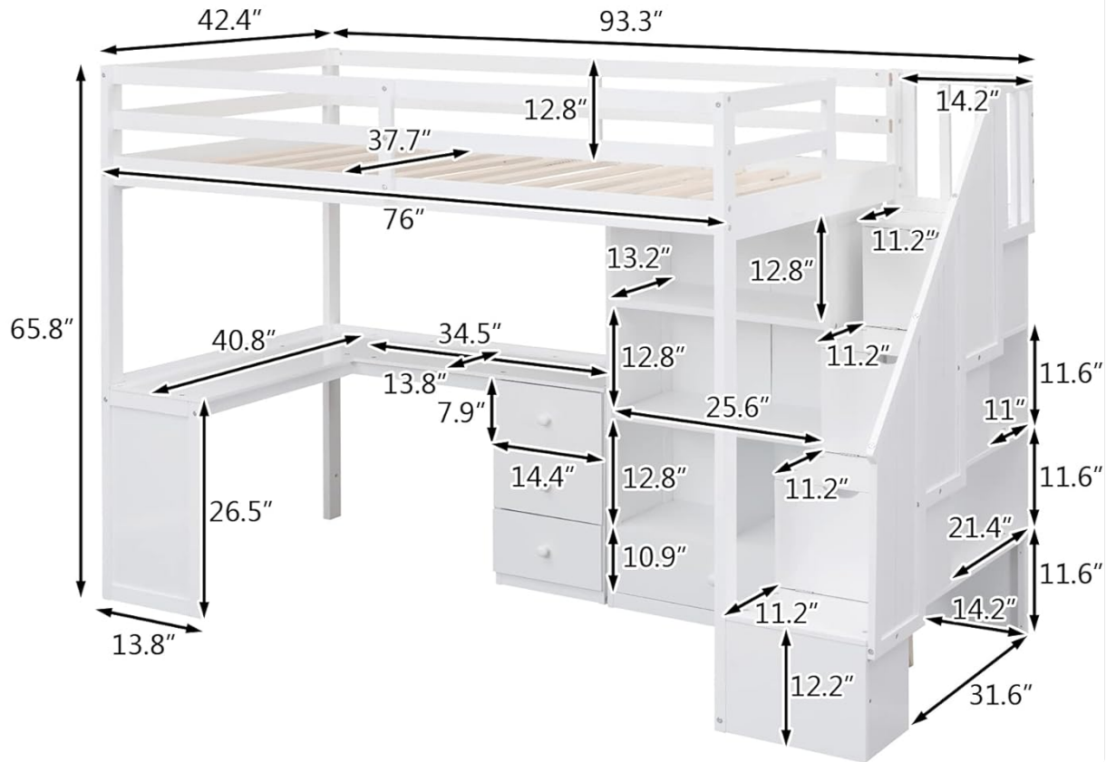
Image 7.1: A technical diagram illustrating the precise dimensions of the SOFTSEA Twin Size Loft Bed, including height, length, and width of various components.
