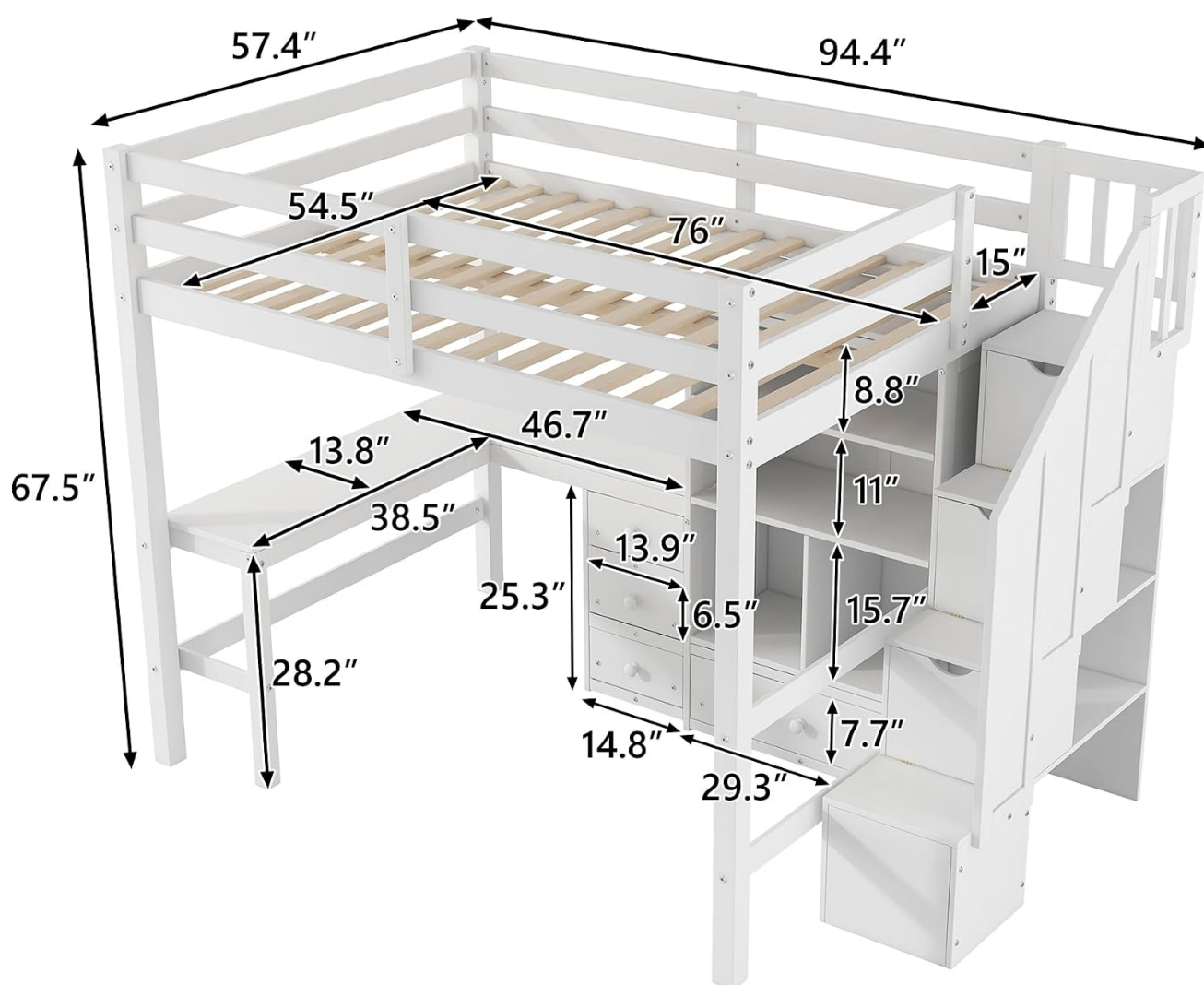
Figure 4.1: Overall Dimensions of the Loft Bed. The bed measures 94.4 inches in length, 57.4 inches in width, and 67.5 inches in height. Detailed measurements for the desk, shelves, and staircase are also provided.
