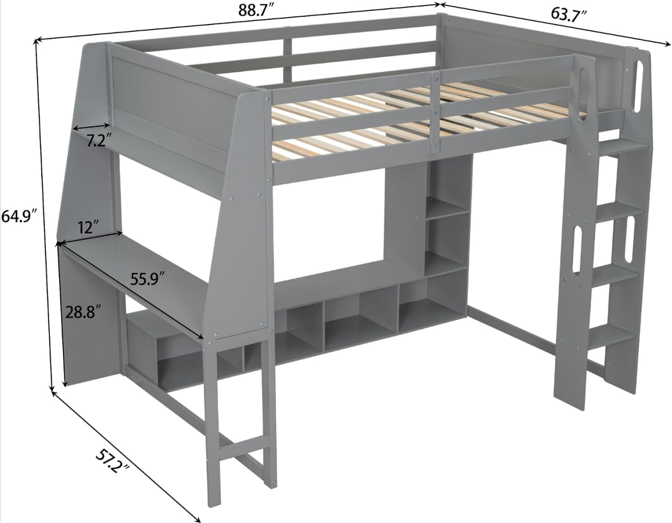
Image 6: Dimensional drawing of the loft bed, providing key measurements for planning and installation.
