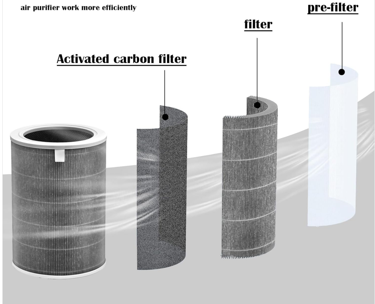
Image: A detailed breakdown of the filter's three layers: pre-filter, main filter, and activated carbon filter.
