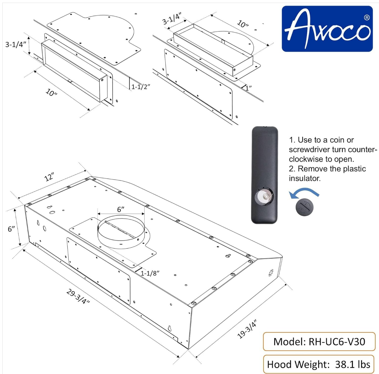
Figure 2: Product dimensions and remote control battery information.
