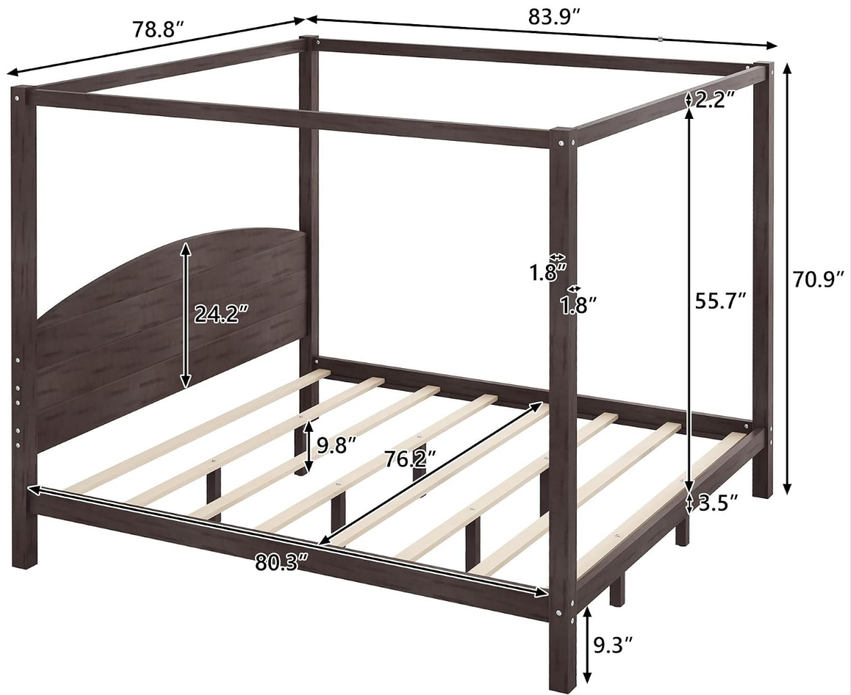
Image: Detailed diagram showing the dimensions of the Merax King Canopy Bed Frame.
