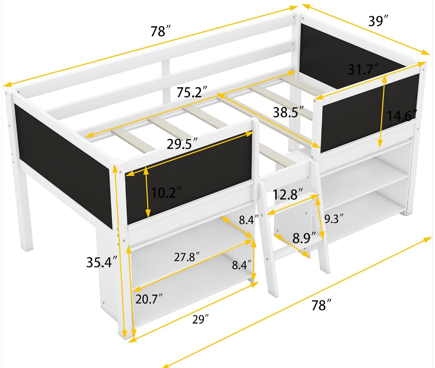
Figure 2: Product Dimensions Overview
