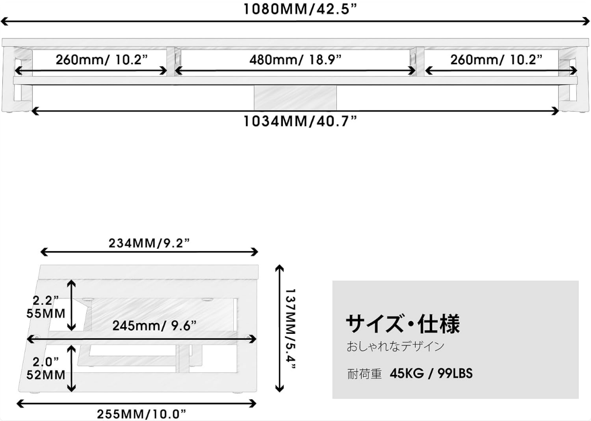
Image 7.1: Detailed dimensions of the Fenge 2-Tier Monitor Stand.
