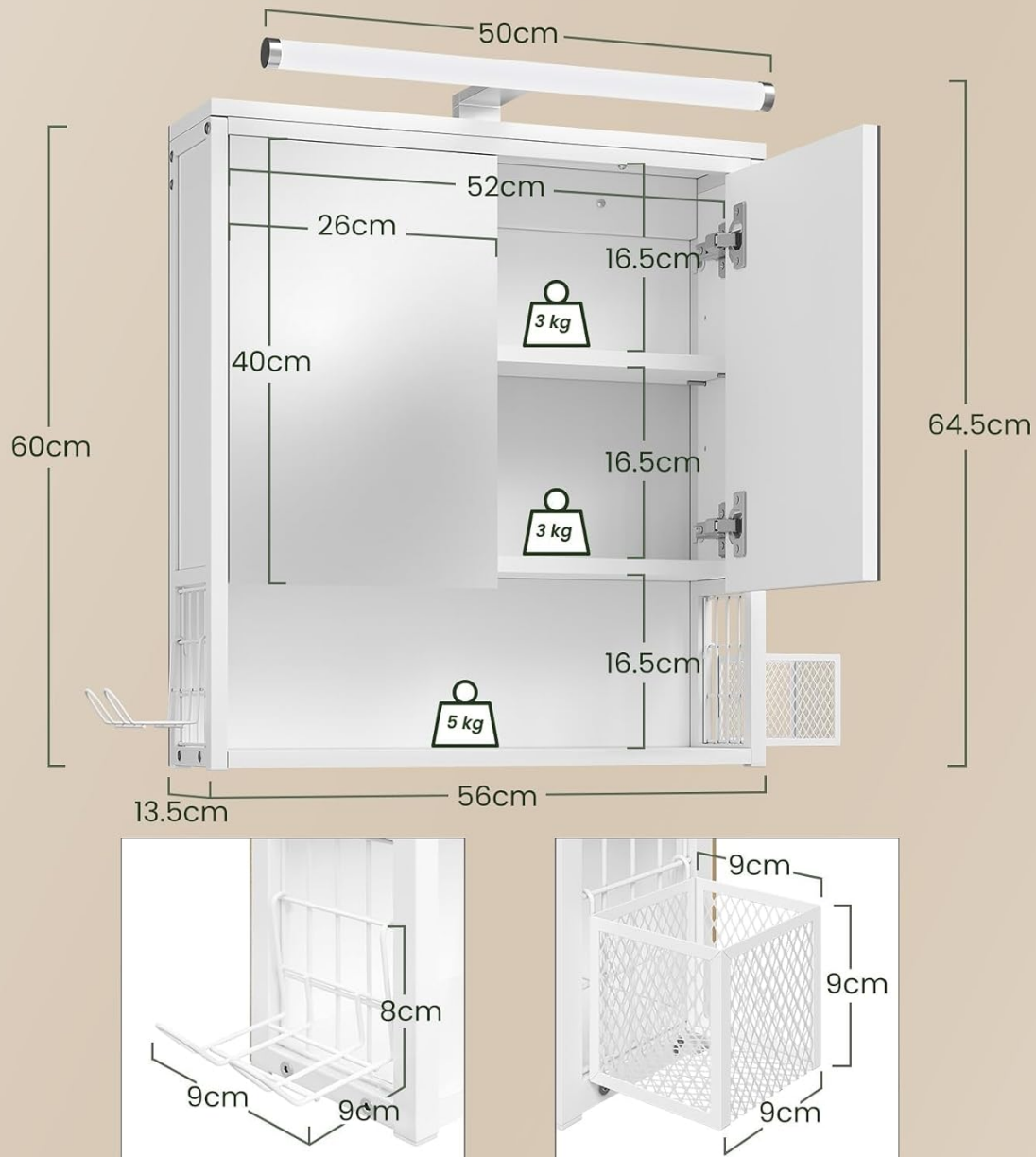
Image 3.1: Technical diagram illustrating the dimensions and load capacities for different sections of the cabinet.
