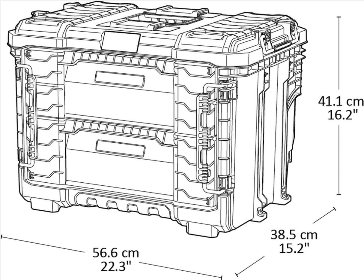
Image: A technical drawing illustrating the dimensions of the Keter Pro Gear XL 2-Drawer Tool Box, showing length, width, and height in both centimeters and inches.
