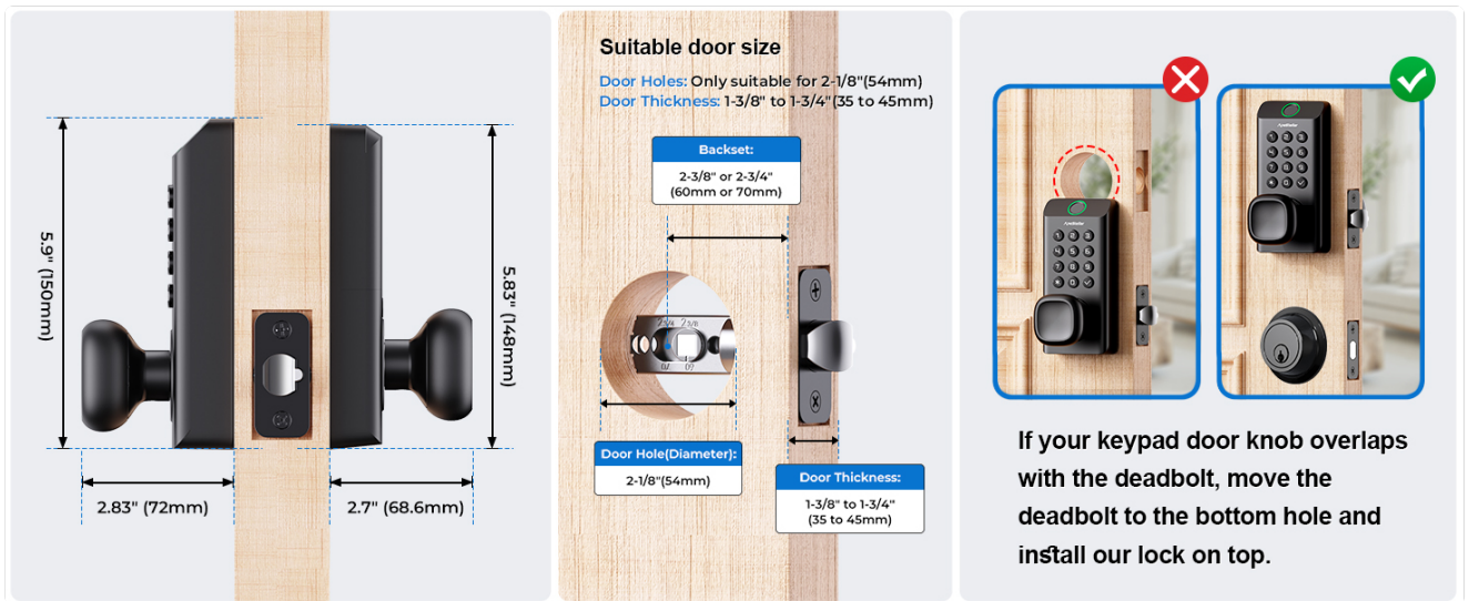
Figure 10: Keypad lockout after multiple incorrect entries.
