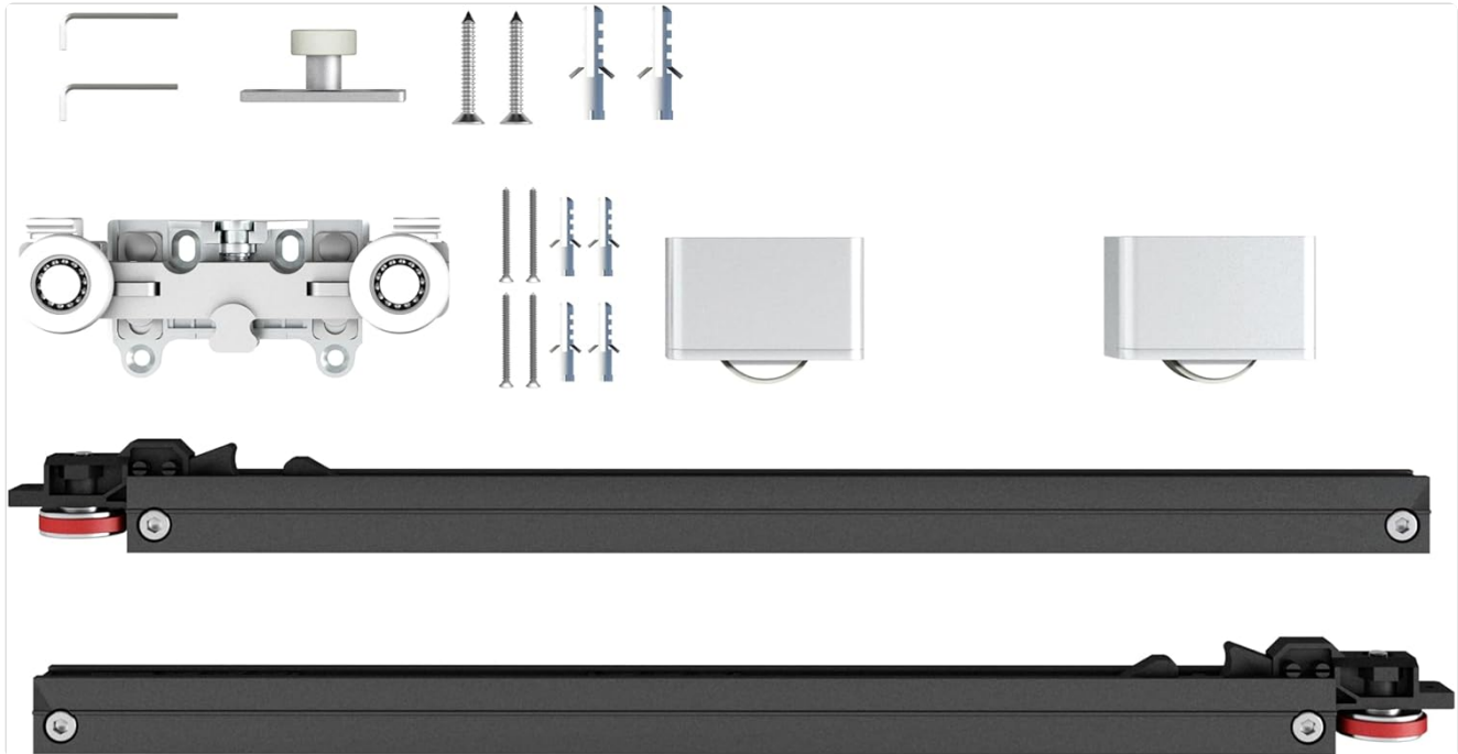
Image 3.1: An overview of the hardware components included in the hidden track system, including rollers, track, and various fasteners.
