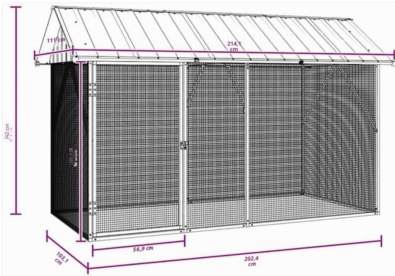
Figure 2: Technical diagram showing the dimensions of the aviary. Total length is 202.4 cm (79.7 inches), total depth is 103.1 cm (40.6 inches), and total height at the peak is 142 cm (55.9 inches).
