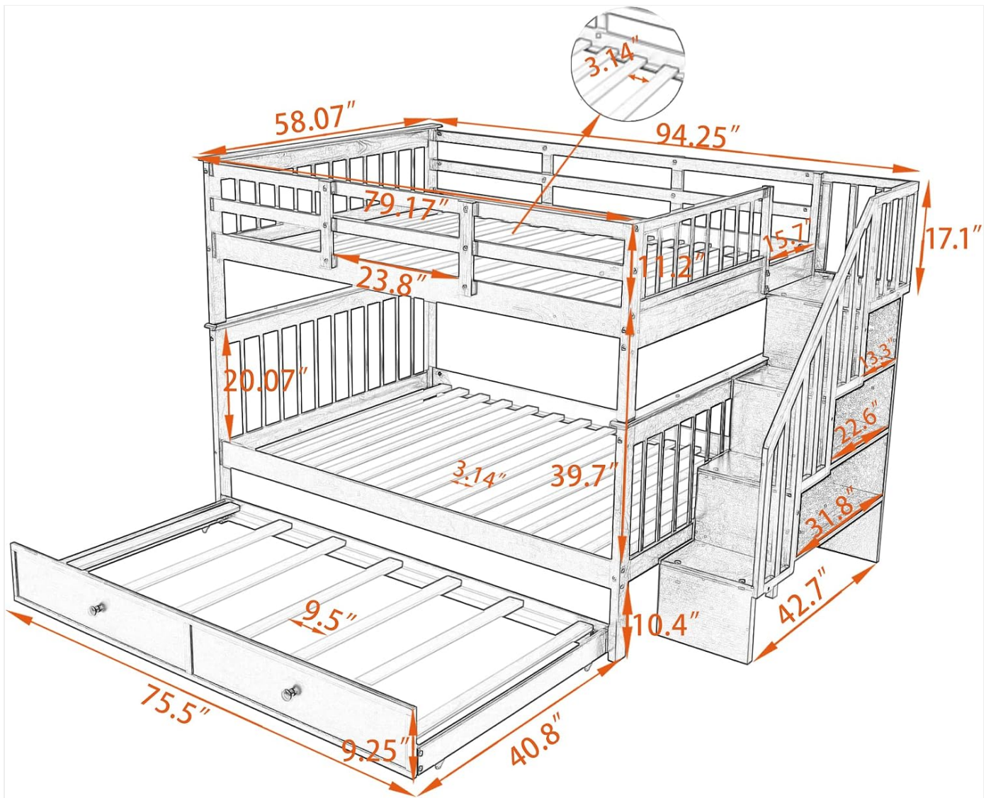
Image 2: Technical drawing illustrating the overall dimensions and key measurements of the bunk bed and trundle unit.
