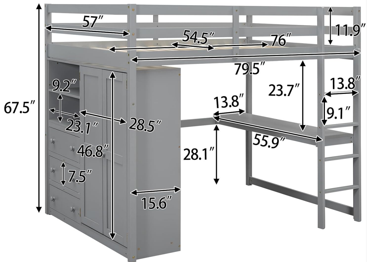
Figure 2: Detailed dimensions of the LIFE SKY Full Luxurious Loft Bed, including bed frame, desk, and wardrobe measurements.
