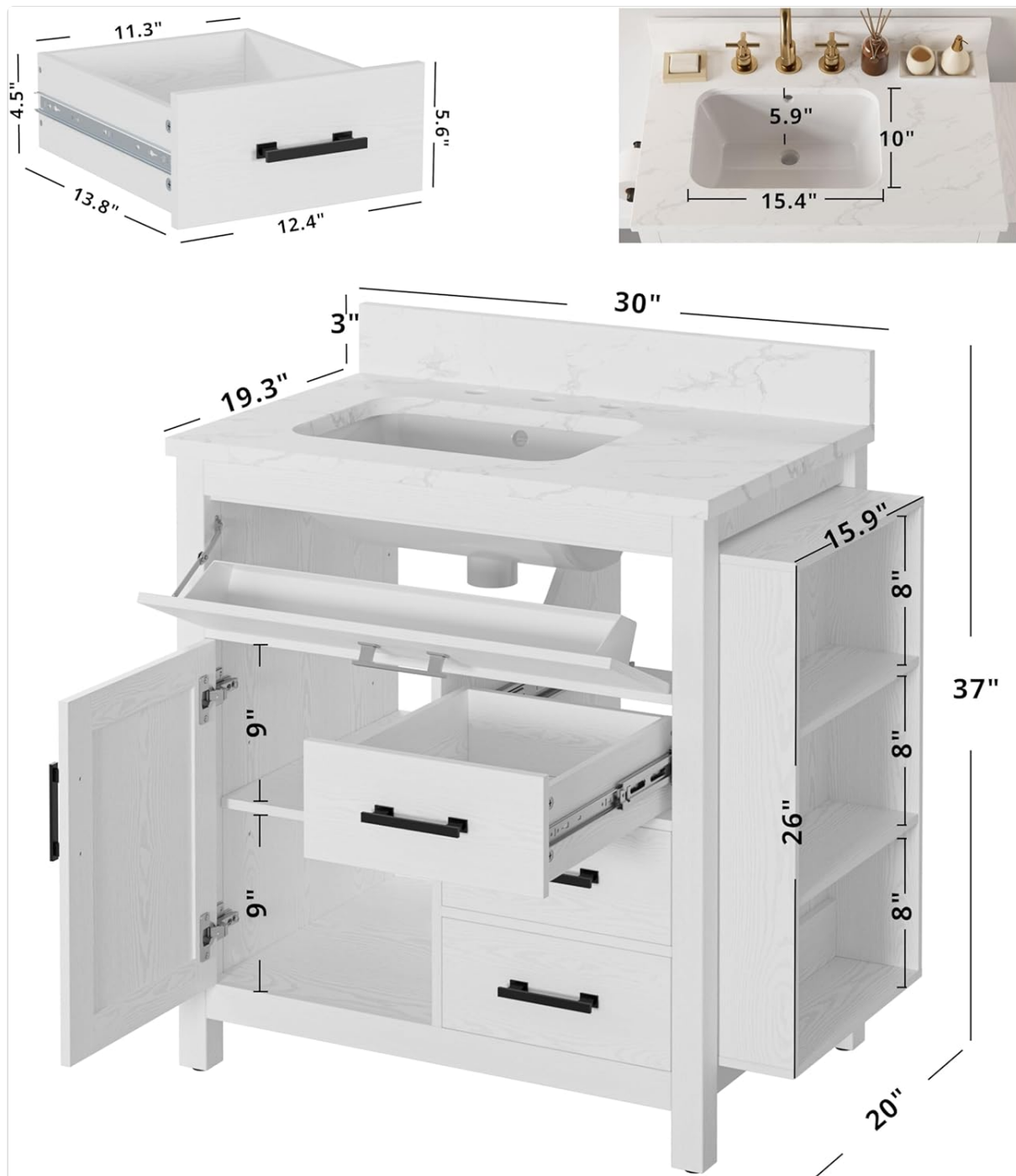
Image 2.2: Diagram showing the detailed dimensions of the vanity, sink, and drawers.
