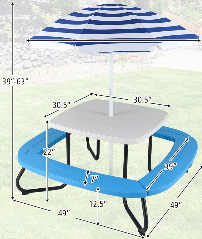
Figure 2: Product dimensions and weight capacities.
