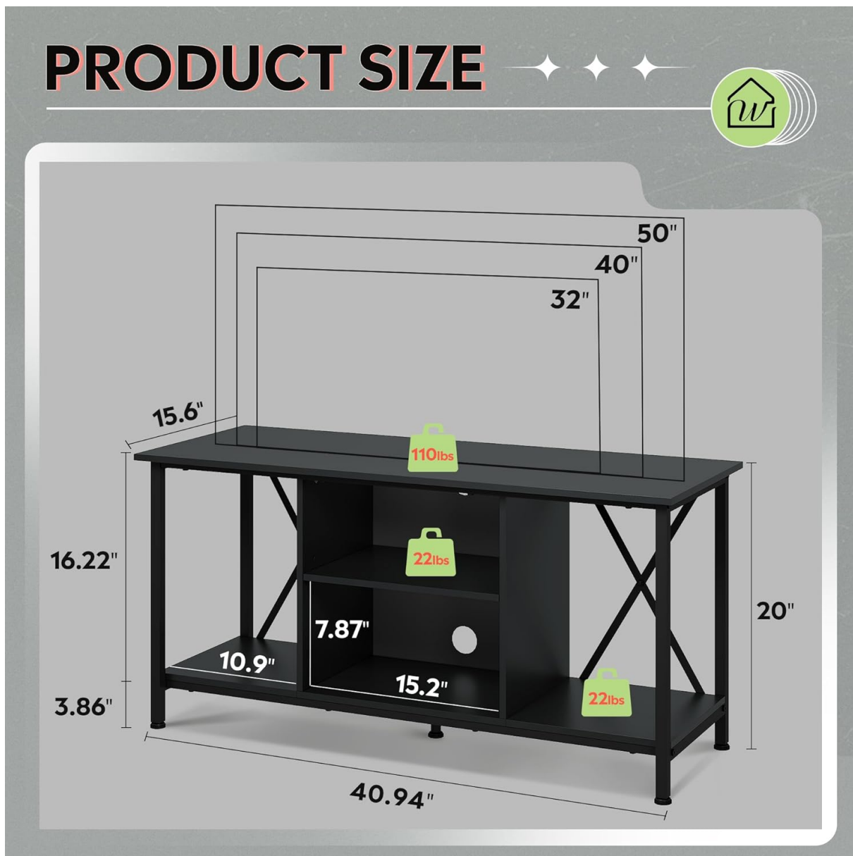
Image 8.1: Detailed product dimensions and weight capacities for the 41-inch TV stand.
