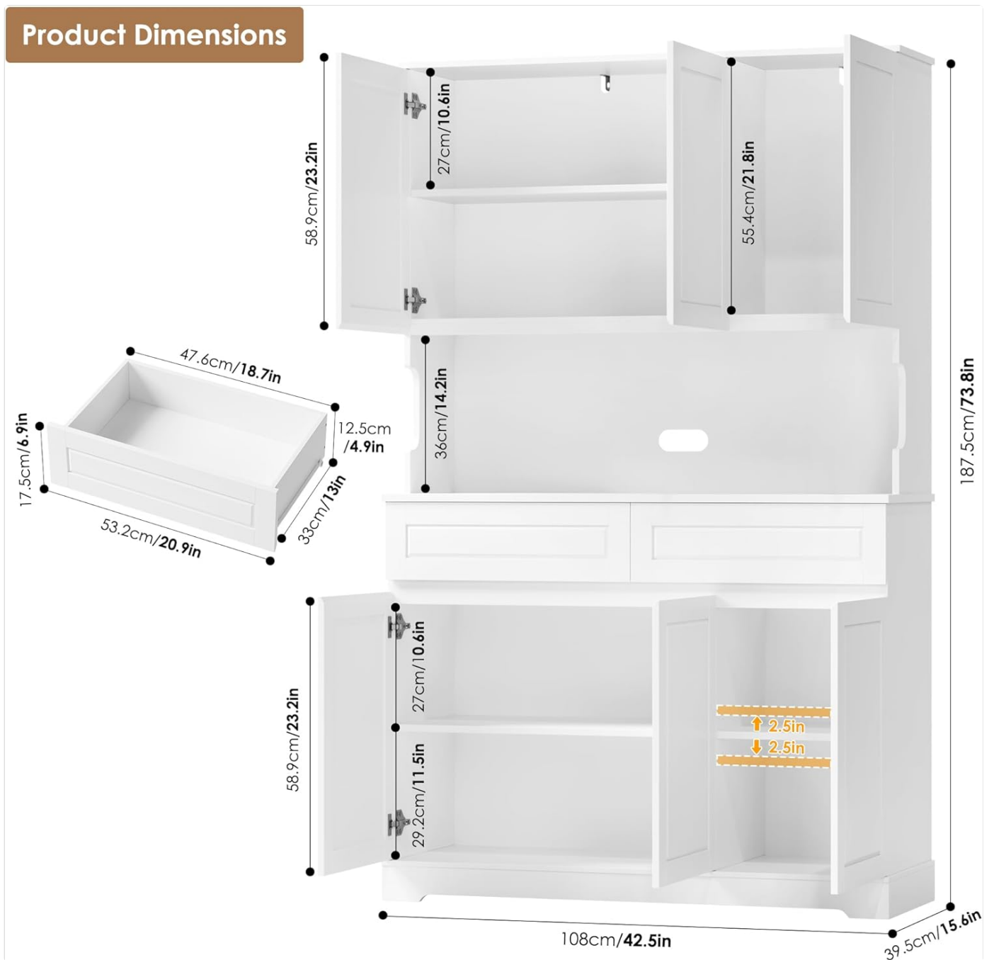
Image 8.1: Diagram illustrating the precise dimensions of the pantry cabinet and its internal components.
