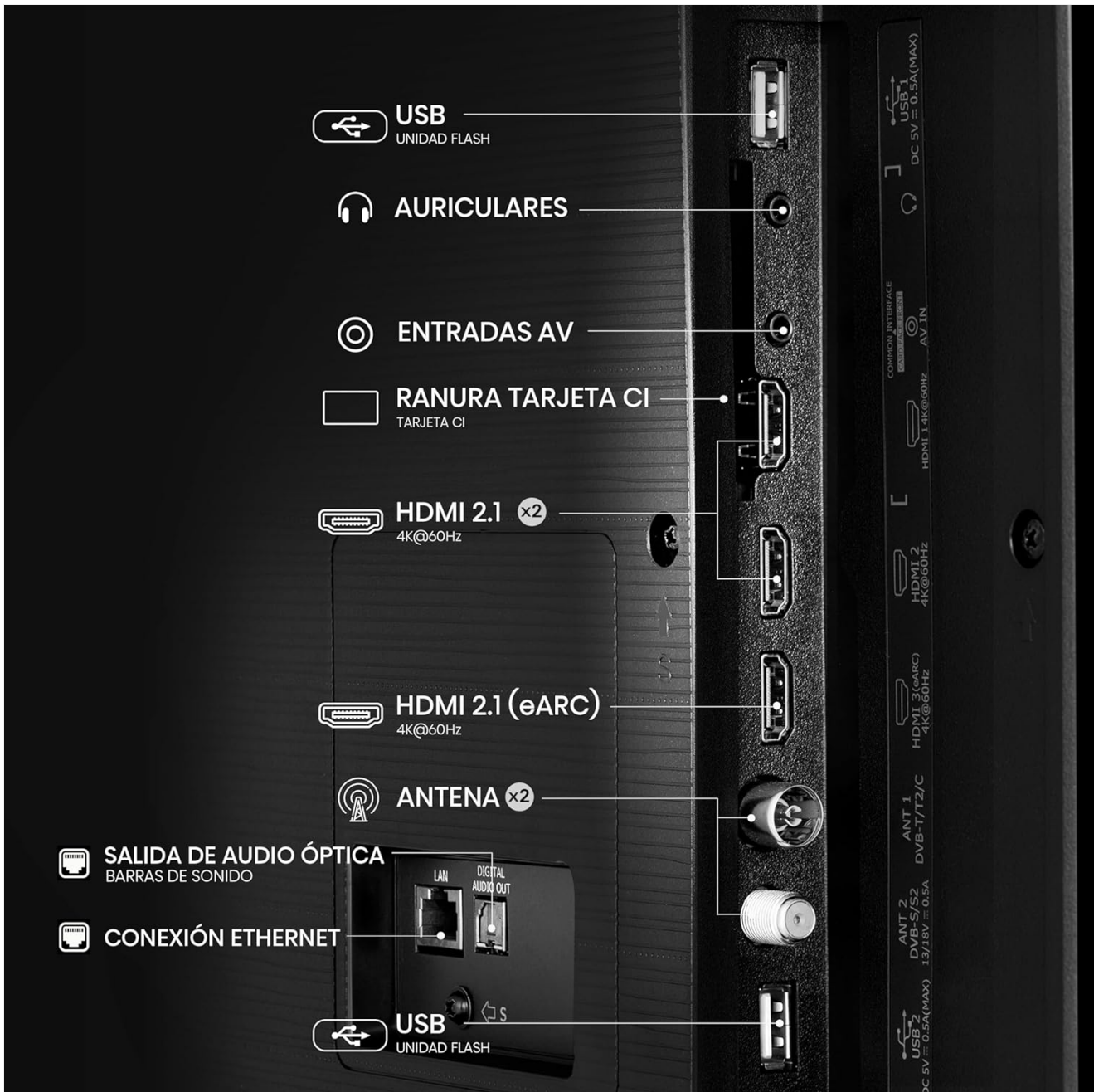
Rear view showing available ports and connections.
