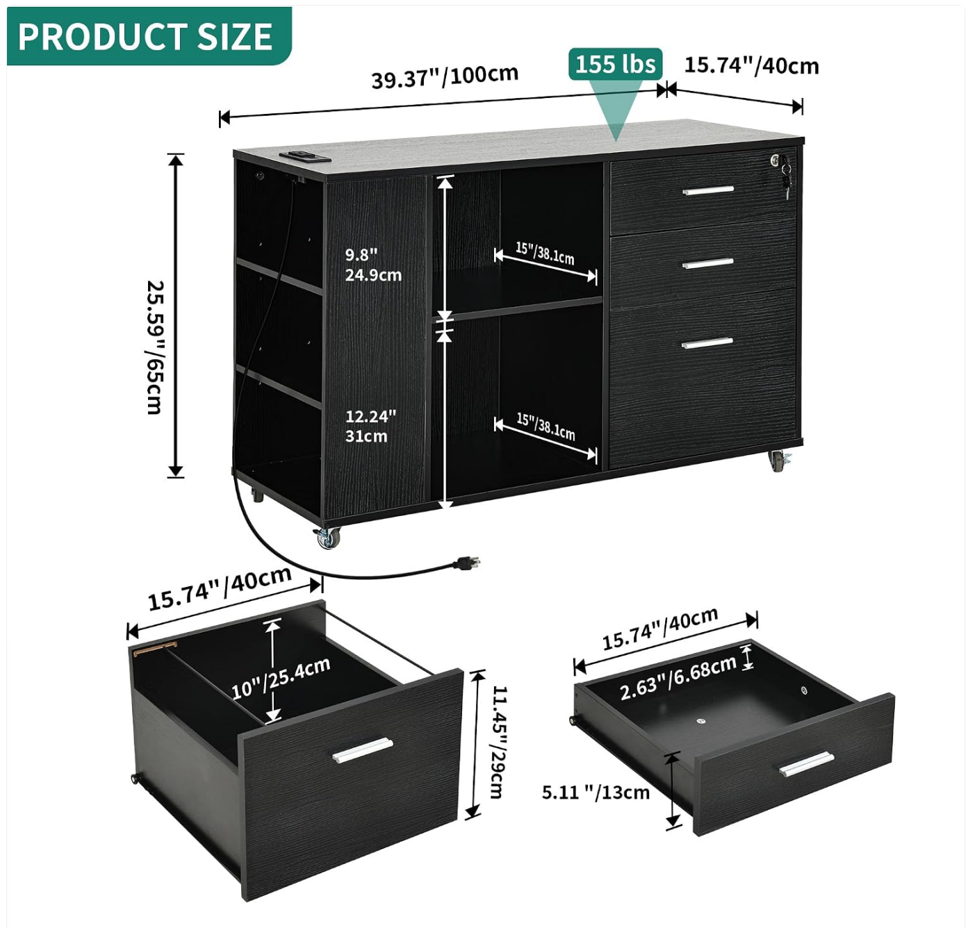
Figure 2: Overview of product dimensions and key structural components.
