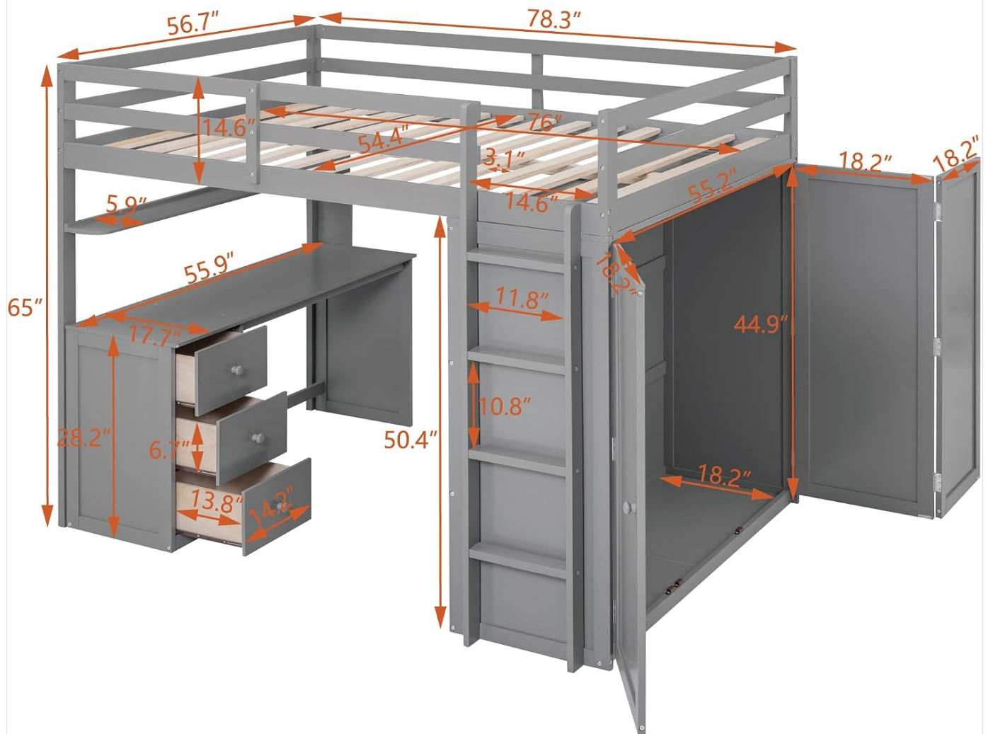
Figure 1: Overall Dimensions of the Loft Bed. This diagram illustrates the complete measurements of the loft bed, including the bed platform (78.3"L x 56.7"W), the desk area (55.9"L x 17.7"W x 28.2"H), and the wardrobe (18.2"W x 44.9"H x 18.2"D), along with the ladder and shelf dimensions.
