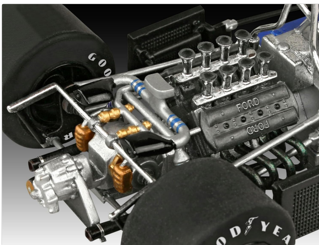
Image: A detailed view of the engine assembly within the Tyrrel P34/2 model, highlighting the intricate components and exhaust system.
