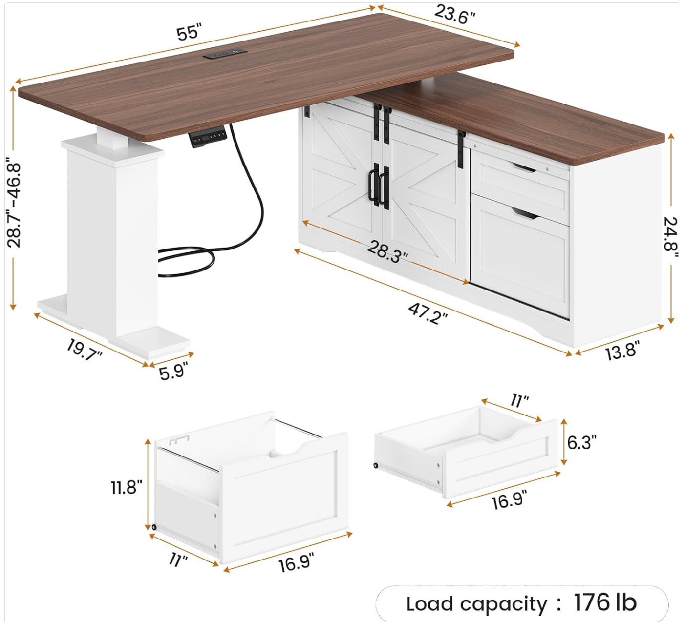
Figure 1: Desk Dimensions and Load Capacity. This diagram illustrates the overall dimensions of the desk, including the main desktop, the L-shaped extension, and the internal storage components. It also specifies the maximum load capacity of 176 lbs.
