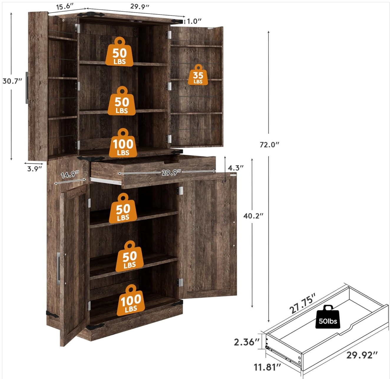
Figure 1: Detailed dimensions and weight capacities of the GRUSIGN storage cabinet.
