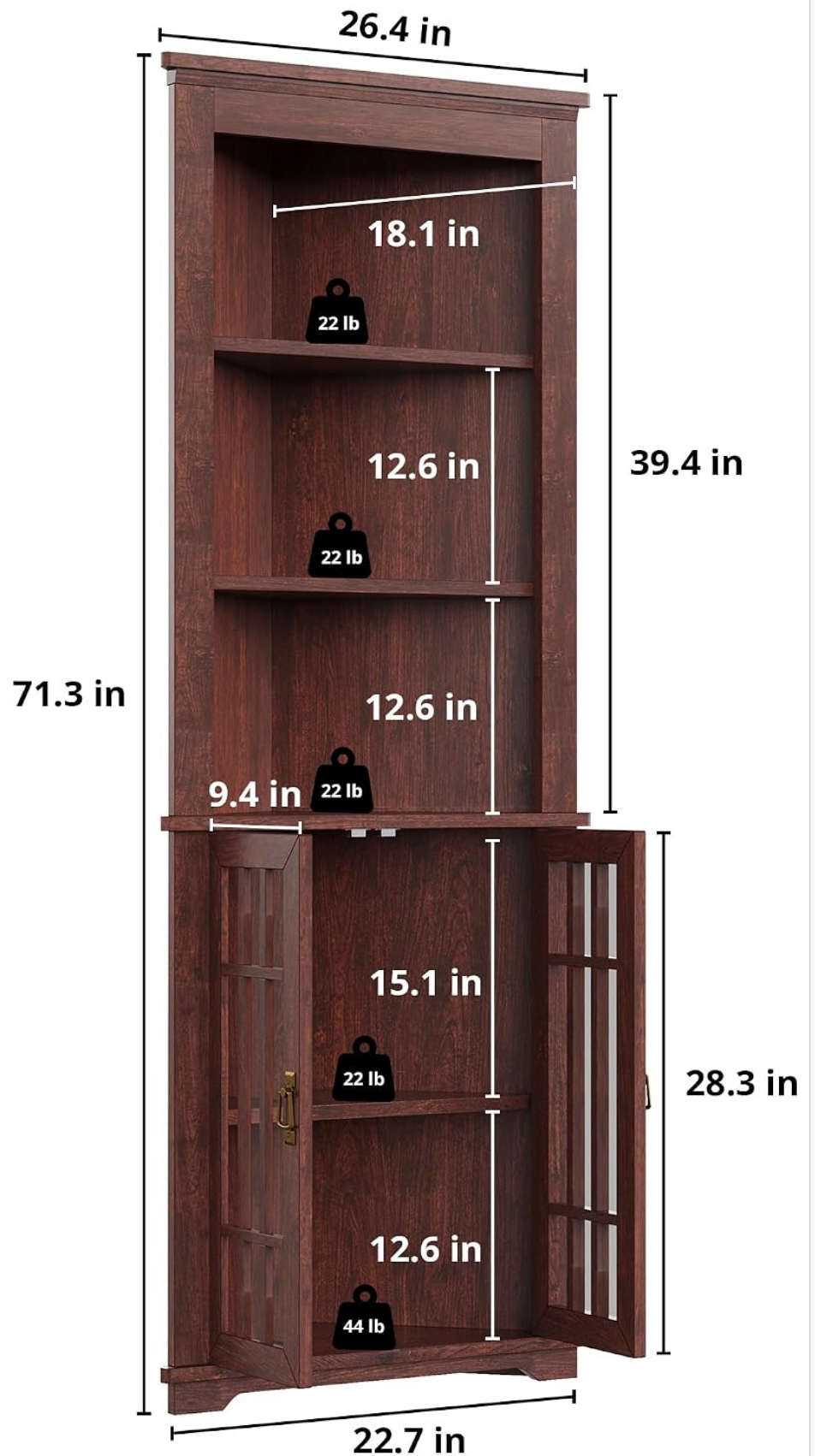
Image: Product dimensions and individual shelf weight capacities.
