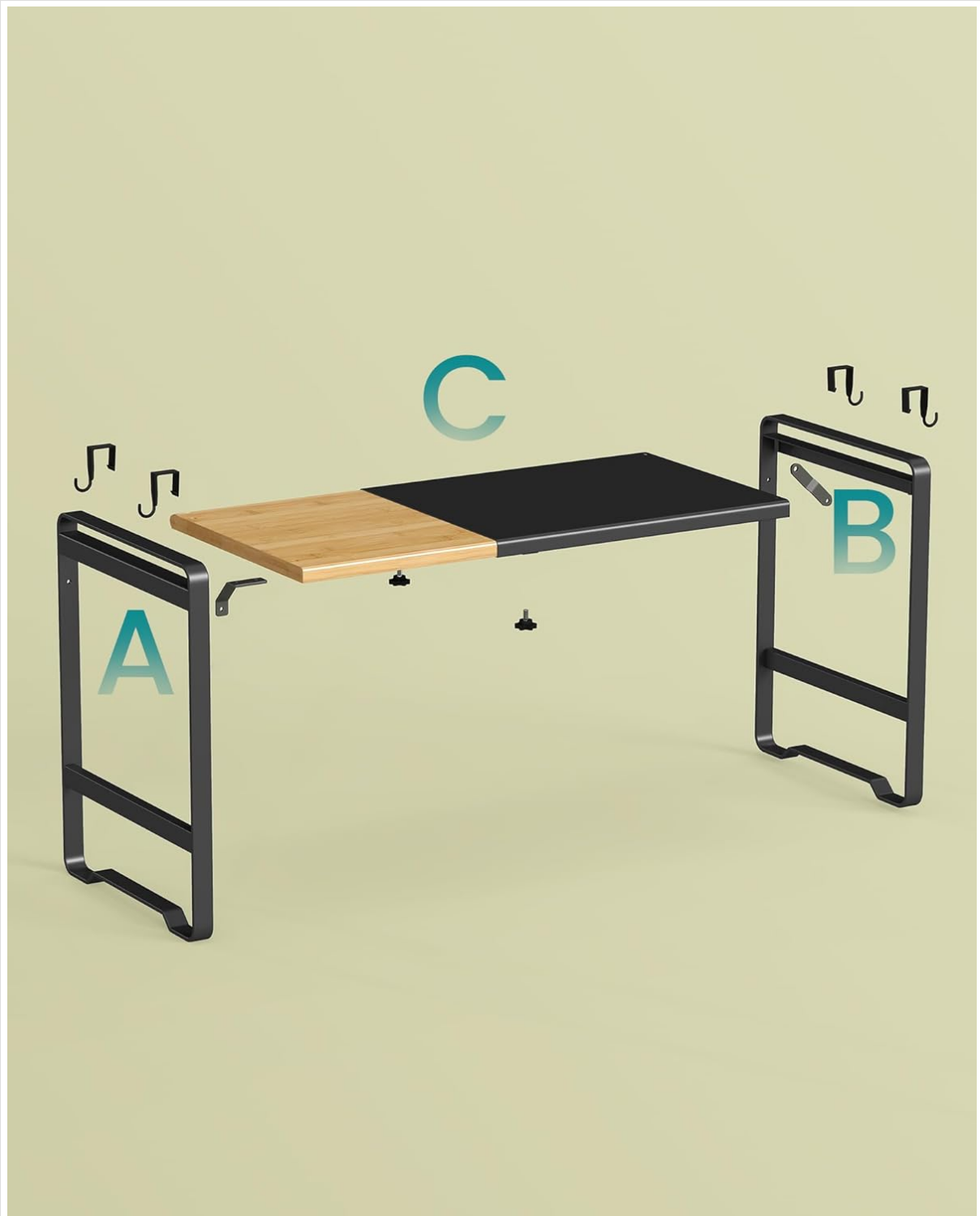
Figure 1: Exploded view of the microwave shelf components, showing side frames (A, B) and the main shelf panel (C) with hooks.
