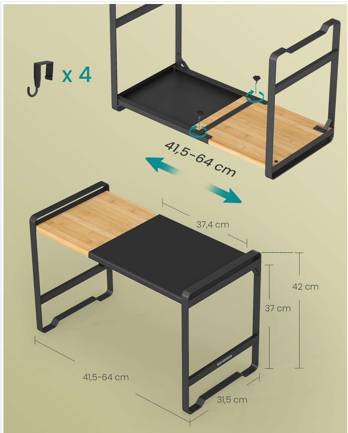
Figure 2: Illustration of the adjustable width feature (41.5-64 cm) and overall dimensions of the assembled shelf.
