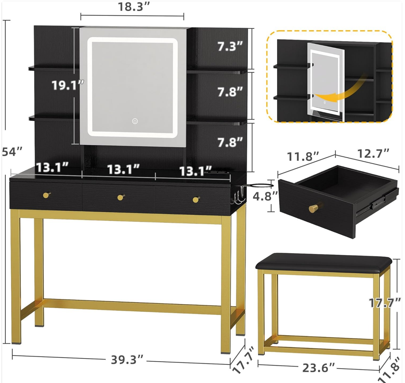
Figure 6: Detailed dimensions of the vanity desk and accompanying stool.
