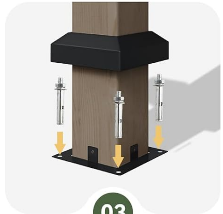
Wind resistance with expansion bolts up to 64-73mph
